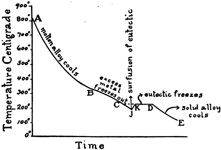
Fig. 15. Surfusions of a Eutectic in a Tin-copper Alloy Cooling Curve:
